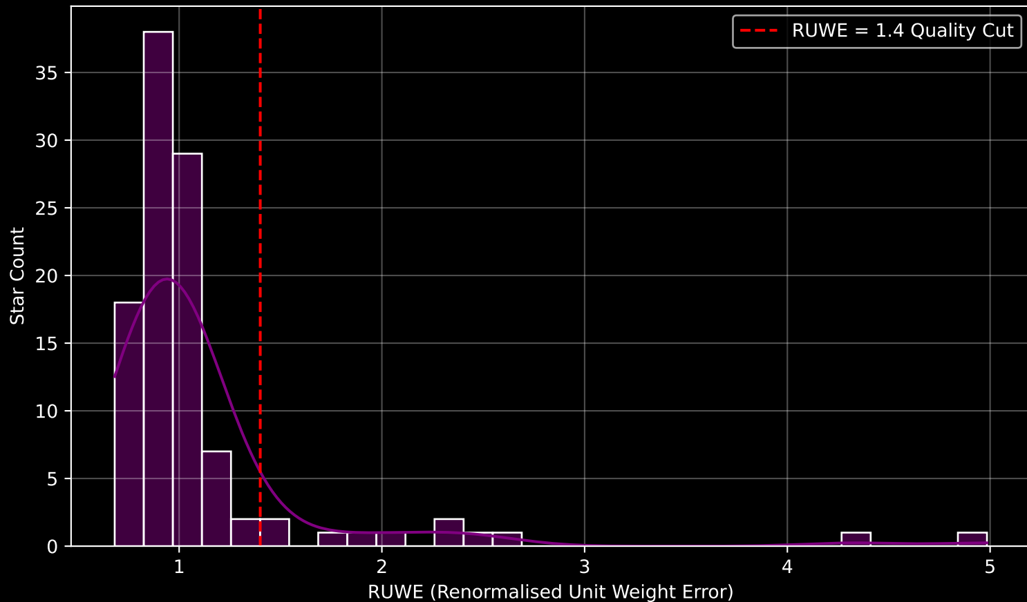
GALAH DR4 Field [7125] RUWE Distribution (n= 105)
