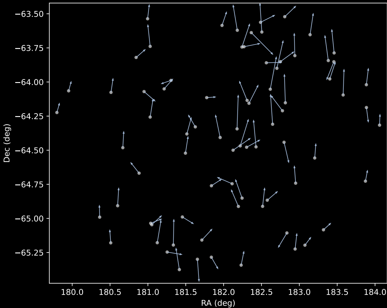
GALAH DR4 Cluster 1 Proper Motion Vectors (n=77)
