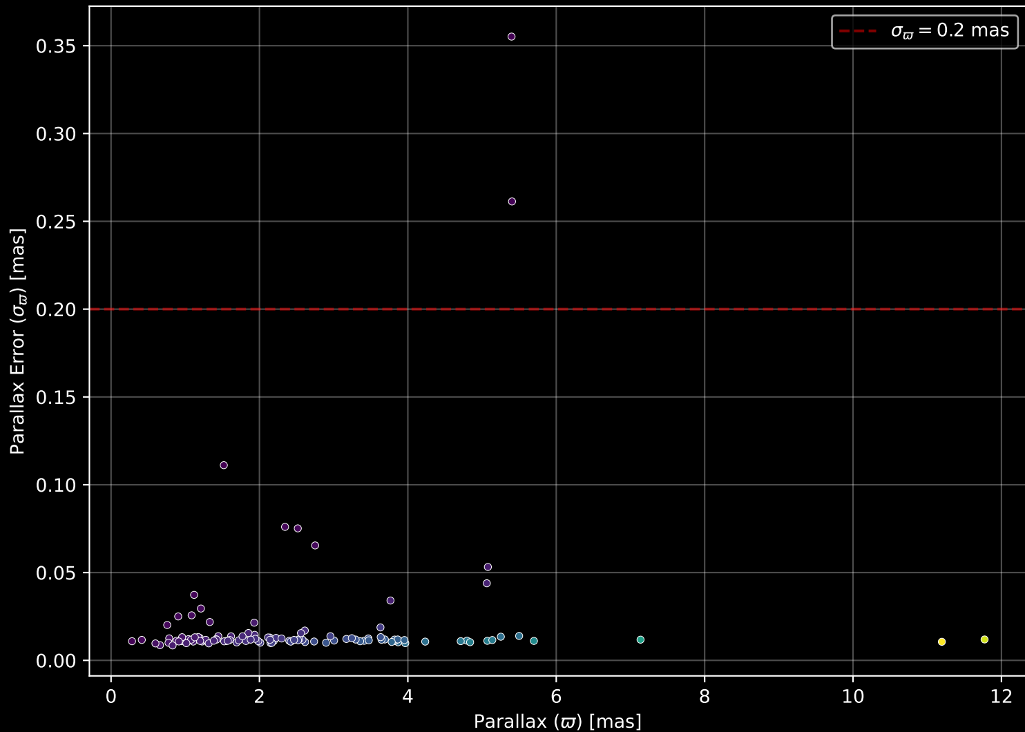
GALAH DR4 Field: [7125] Parallax Quality (n= 110)
