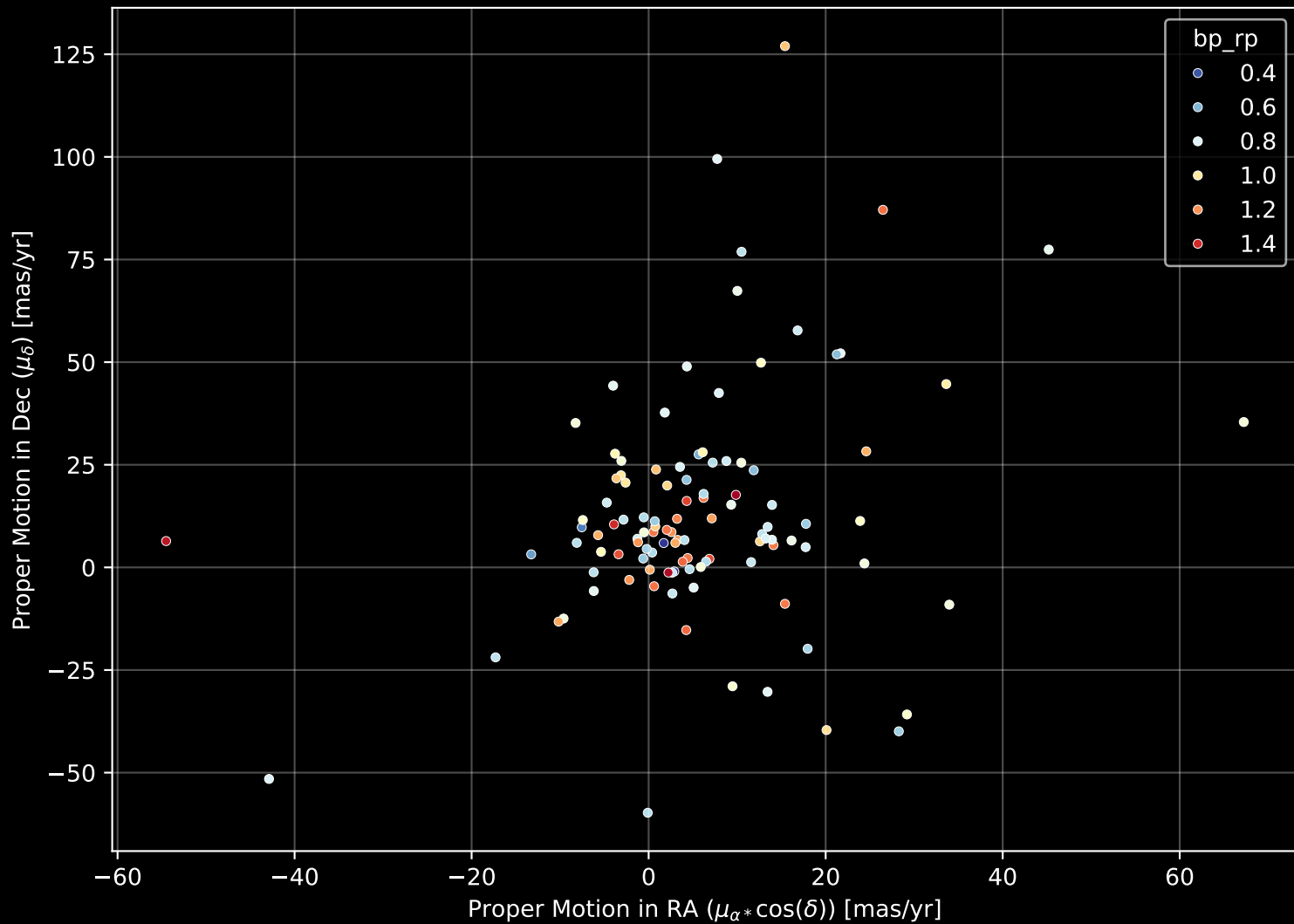
GALAH DR4 Field: [7125] Proper Motion Diagram (n= 110)
