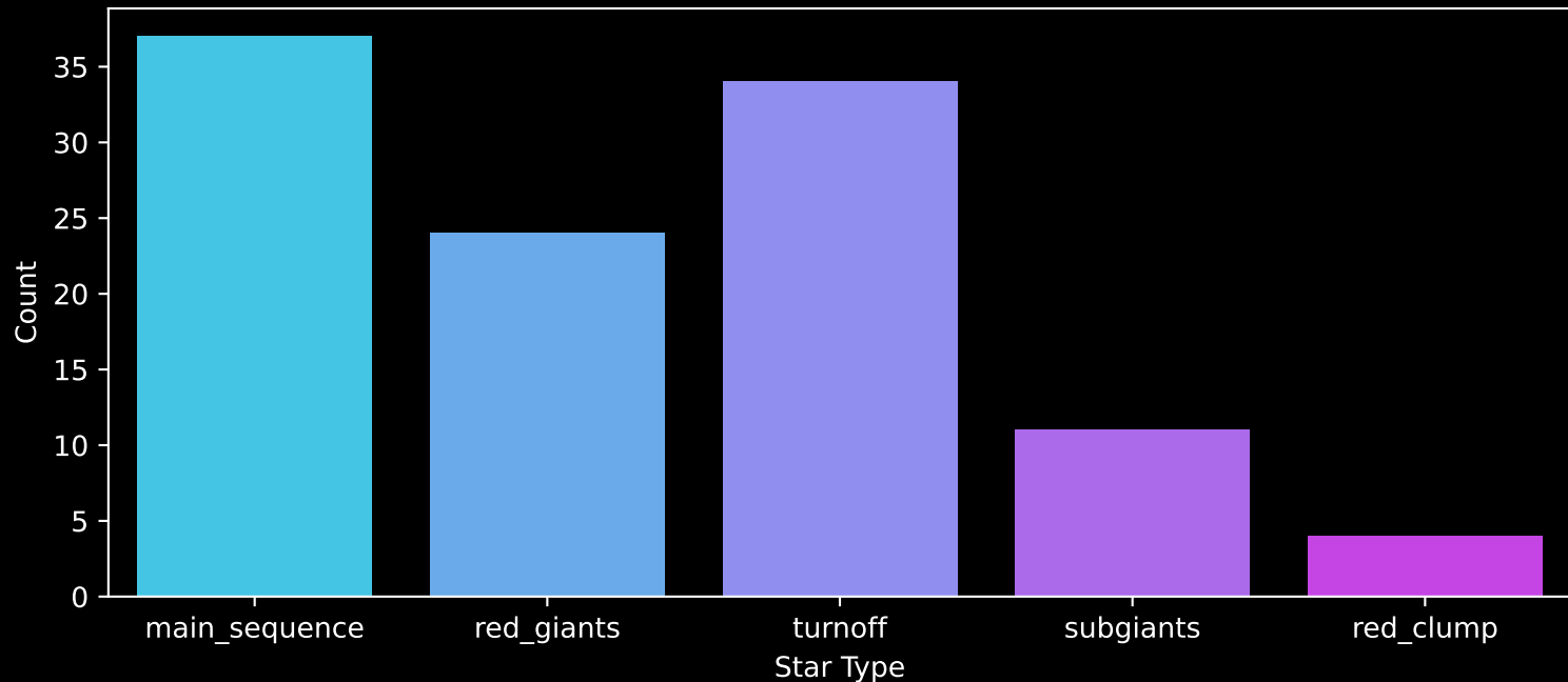
GALAH DR4 Field: [7125] Count plot of Star Type
