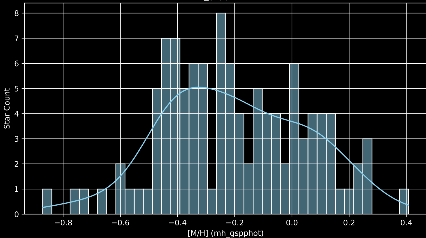
GALAH DR4 Field: [7125] [M/H] (mh_gspphot) (n= 110)
